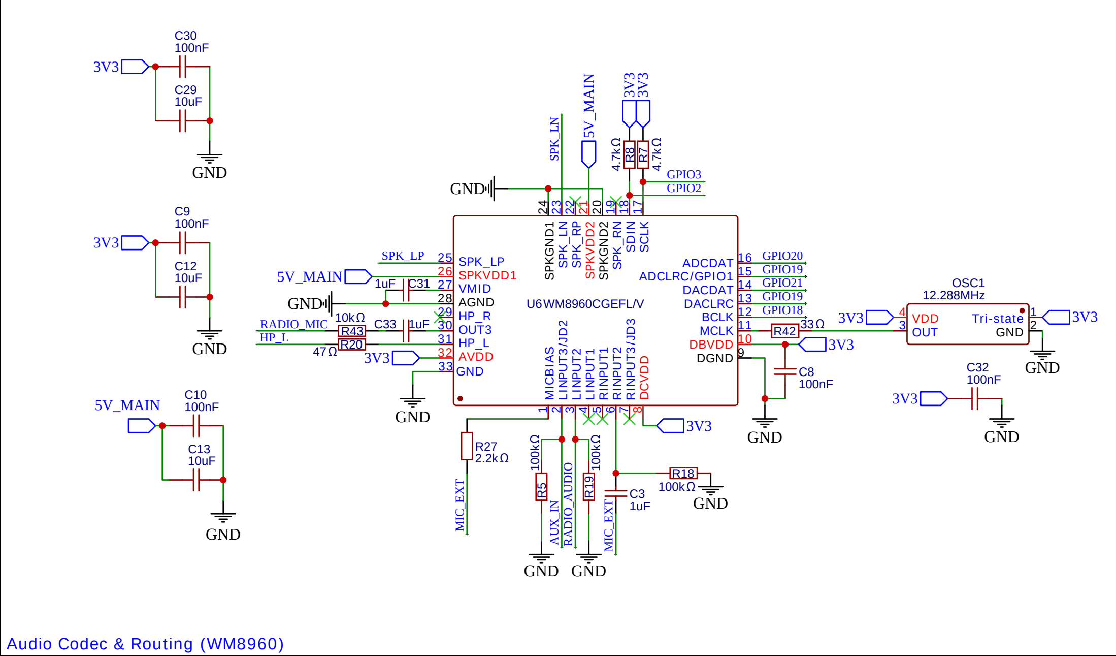
Audio Codec & Routing (WM8960)
