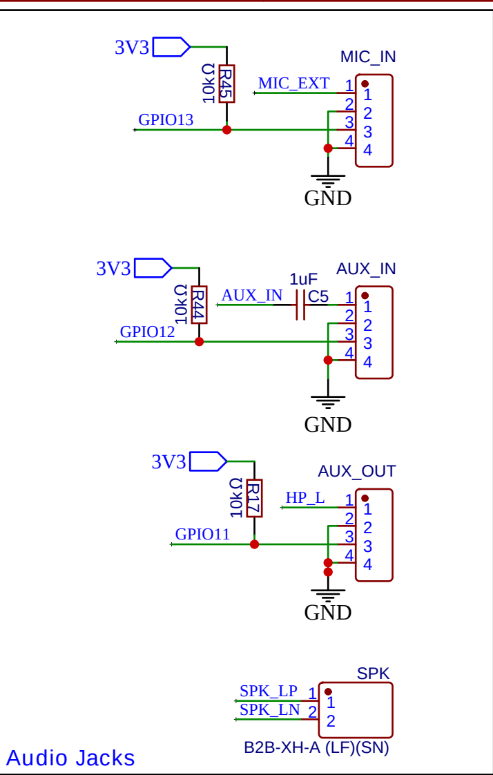
Audio Jacks
