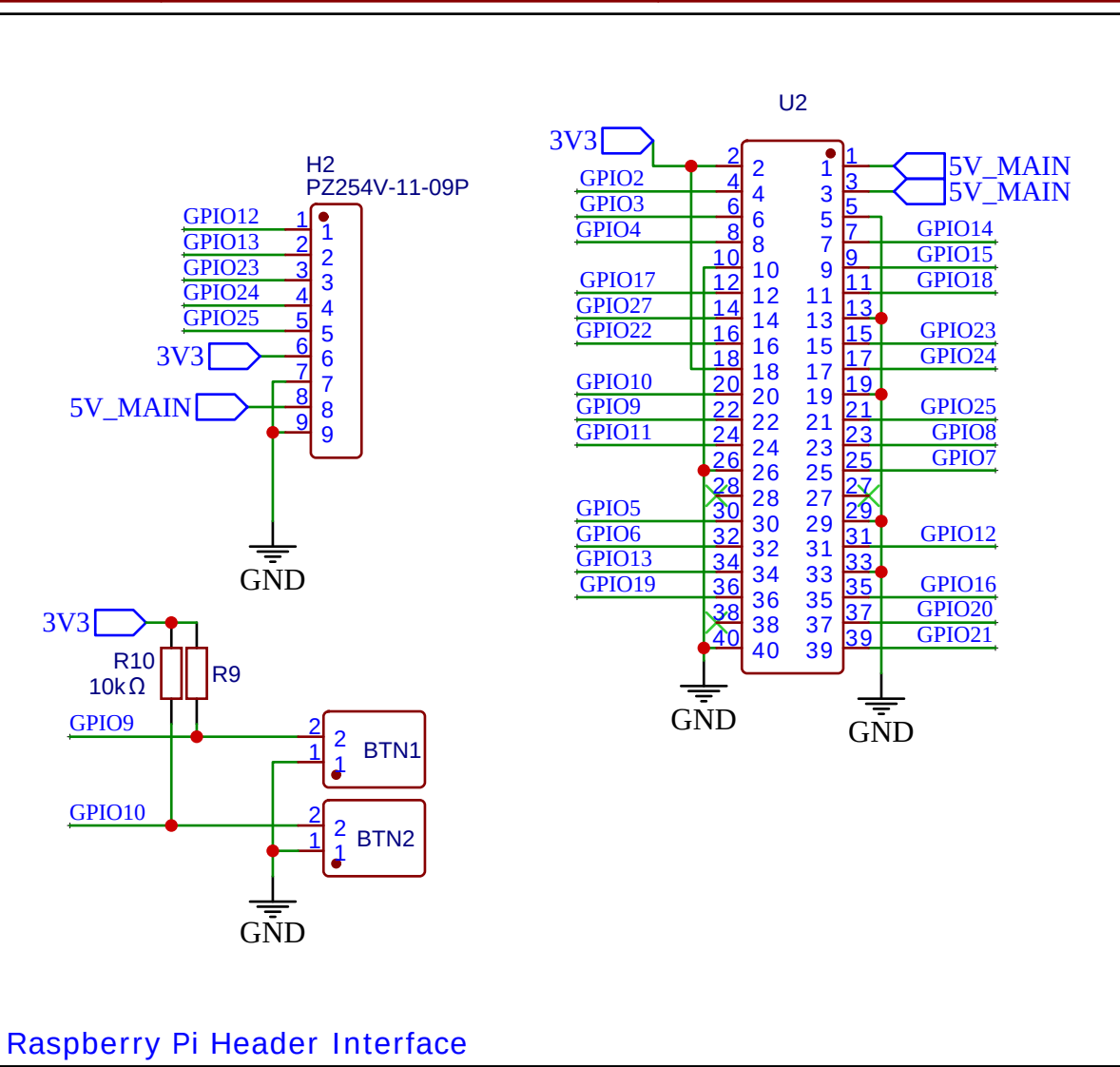
Raspberry Pi Header Interface
