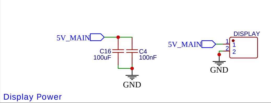
Display Power
