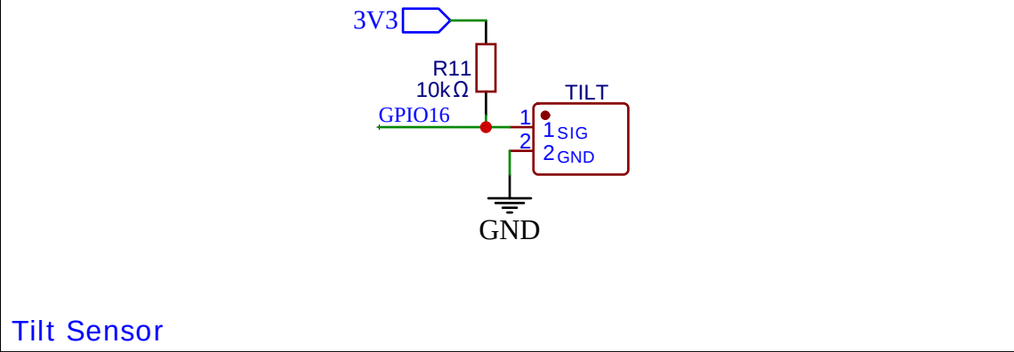
Tilt Sensor
